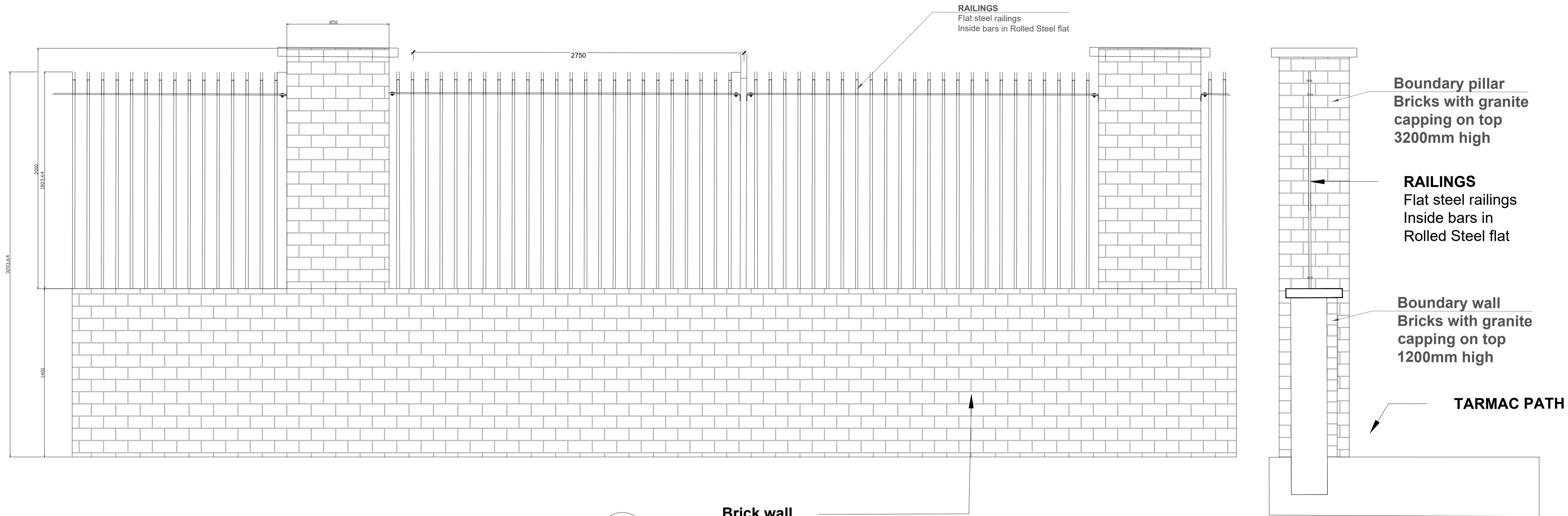
Proposed Boundary wall between Richmond Road phase 2 and the distillery site
